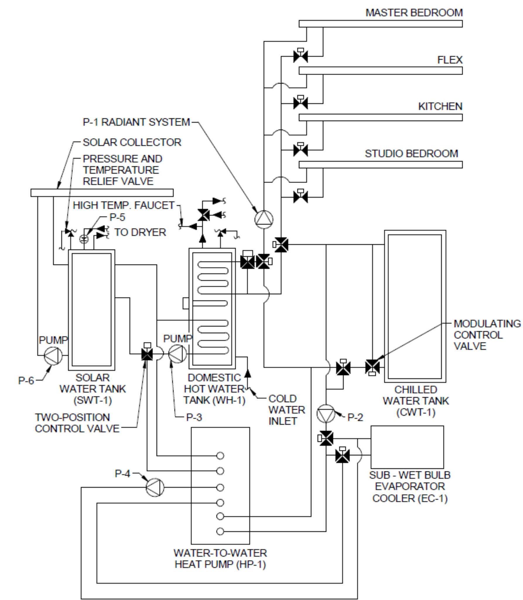
MECHANICAL DIAGRAM
